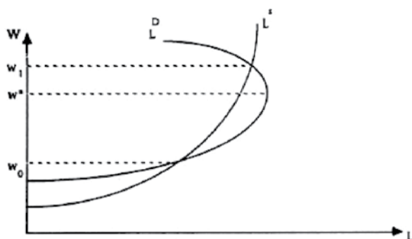
Figure 4-5: Equilibrium in case of several intersection points
