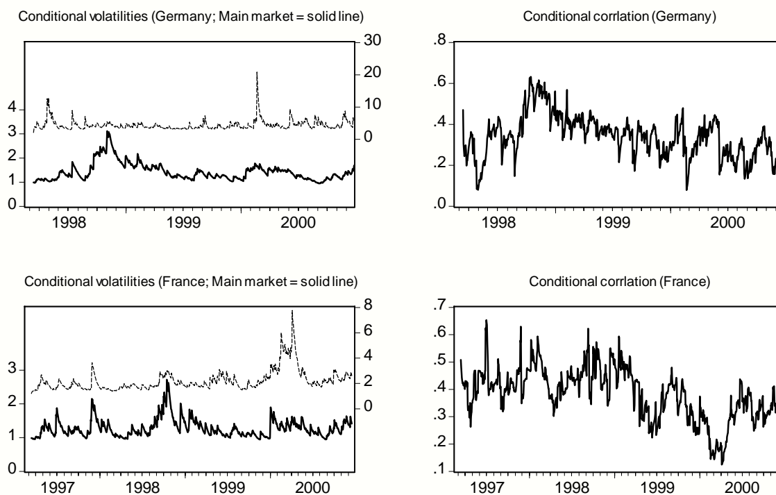
Figure 2 — Estimated Conditional Volatilities and Correlations
