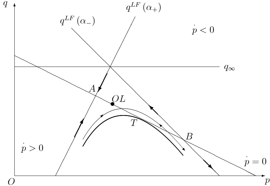
Figure 1 The phase diagram under free trade
