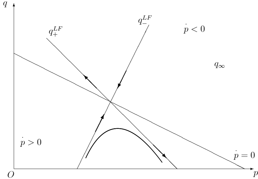
Figure 2 The linear feedback strategies of firm h under the VER
