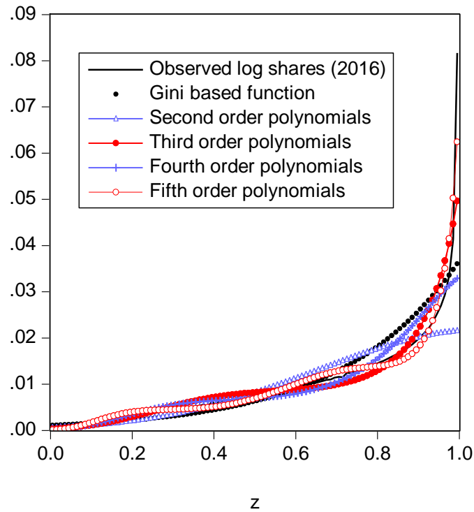
Fig.2 Conver. of Legendre polynomials to obs. log shares
