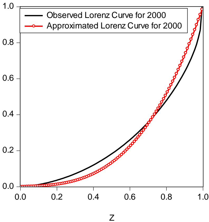
Fig.6 Approximate the Lorenz Curve for 2000
