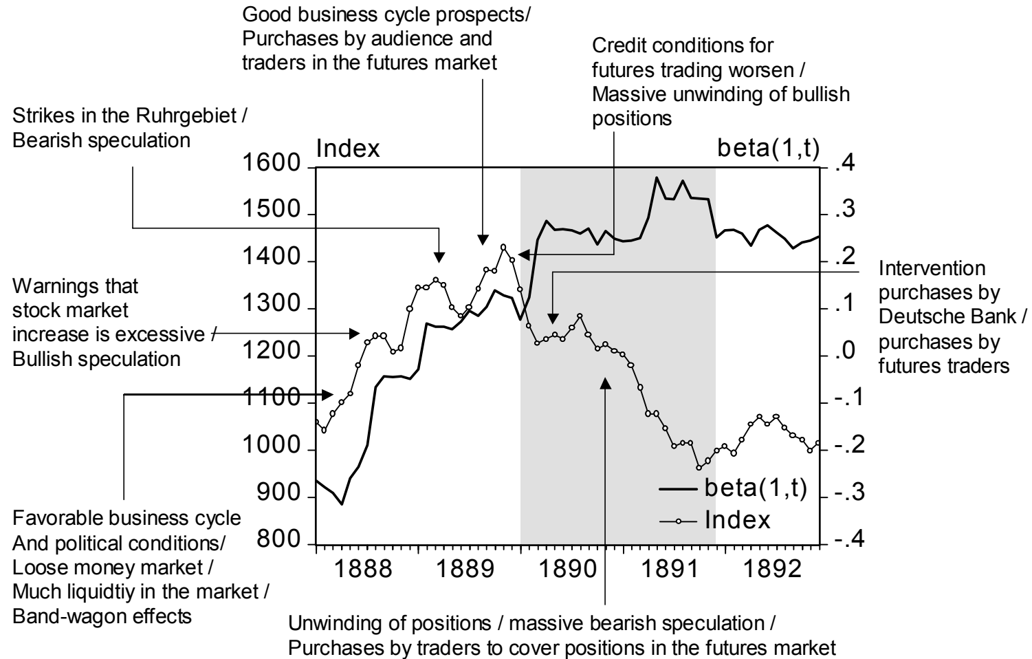
Figure 2: Real stock market index and time-varying return predictability (1888:1 – 1892:12)
