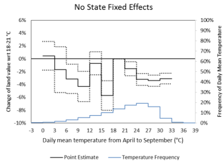
Figure 7. Impact on Northern and Southern regions.
