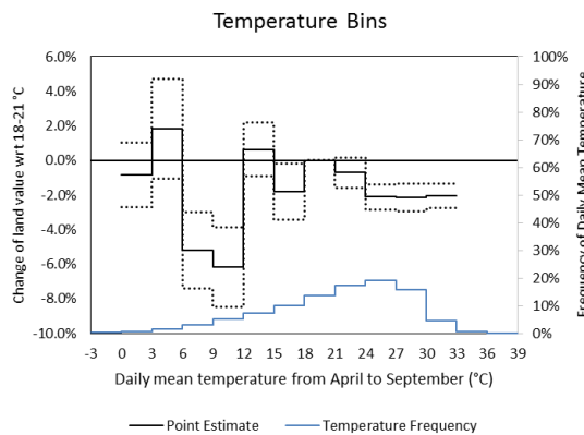
Figure 1. The marginal effect of temperature in the model with average temperature.
