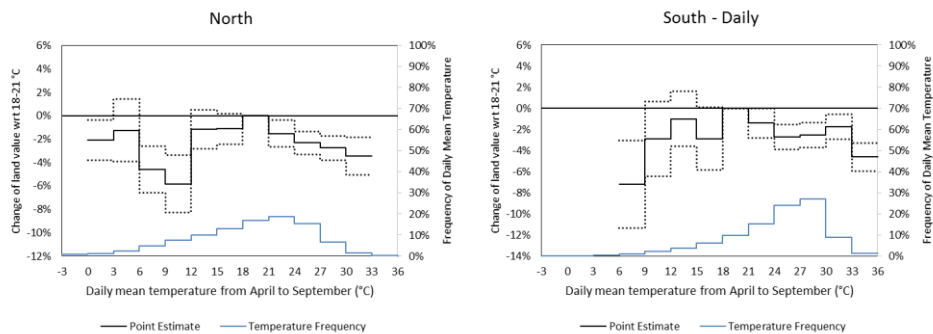
Figure 6. Impacts of daily and monthly temperature on cropland and pastureland.
