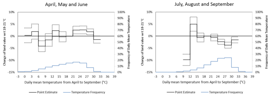
Figure 4. Impact of alternative climate data.
