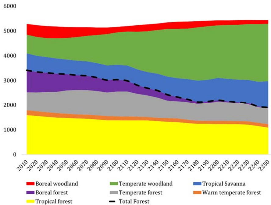
Figure 1: Distribution of potential natural forestland and woodland under the RCP 8.5 scenario (Mha), data from LPX-Bern Global Dynamic Vegetation Model
