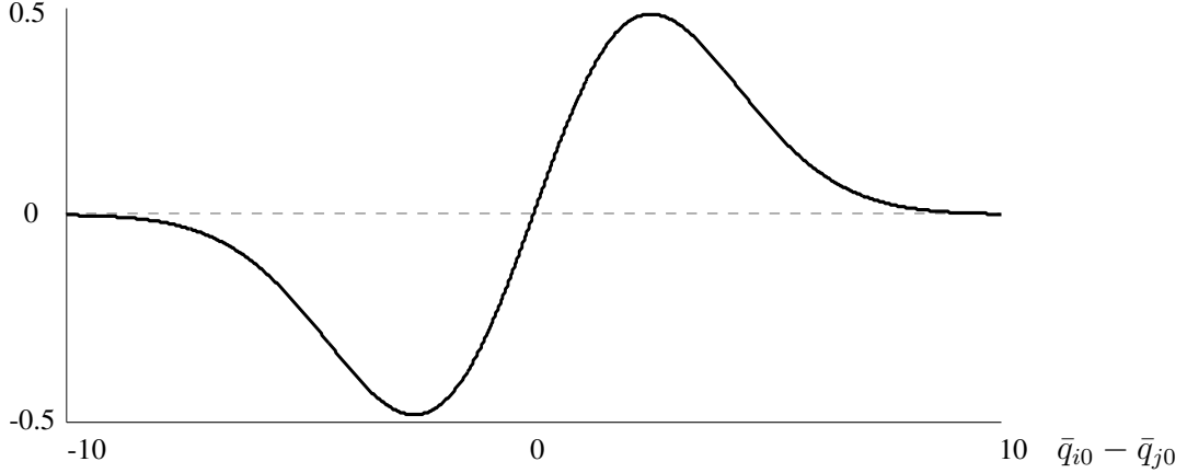
Figure 2: The competition effect in dependence of \bar{q}_{i0} - \bar{q}_{j0} for affine functions for \sigma_{i0}^2 = \sigma_{j0}^2 = \sigma_\varphi^2 = 4 , \beta = 0.5 , \eta_H = 6 , and \eta_L = 2 .
