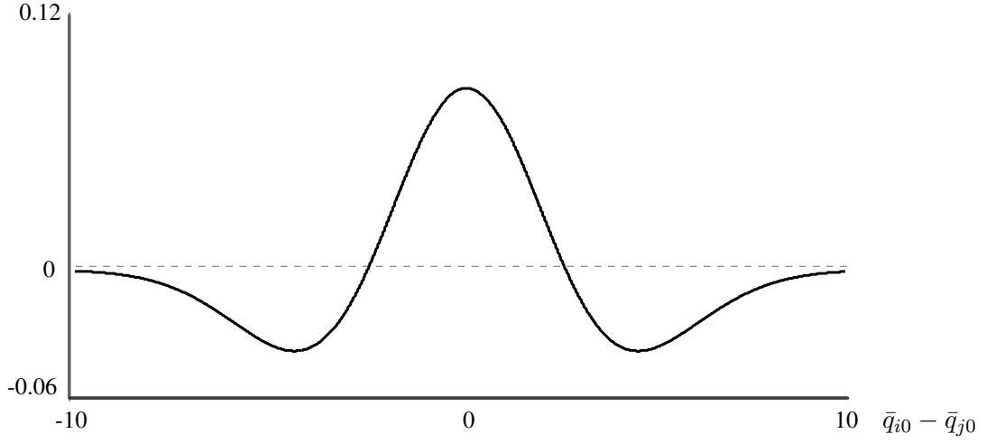
Figure 1: The competition effect in dependence of \bar{q}_{i0} - \bar{q}_{j0} for a constant payoff structure for \sigma_{i0}^2 = \sigma_{j0}^2 = \sigma_{\varphi}^2 = 4 , \beta = 0.5 , \bar{u}_H = 6 , and \bar{u}_L = 2 .
