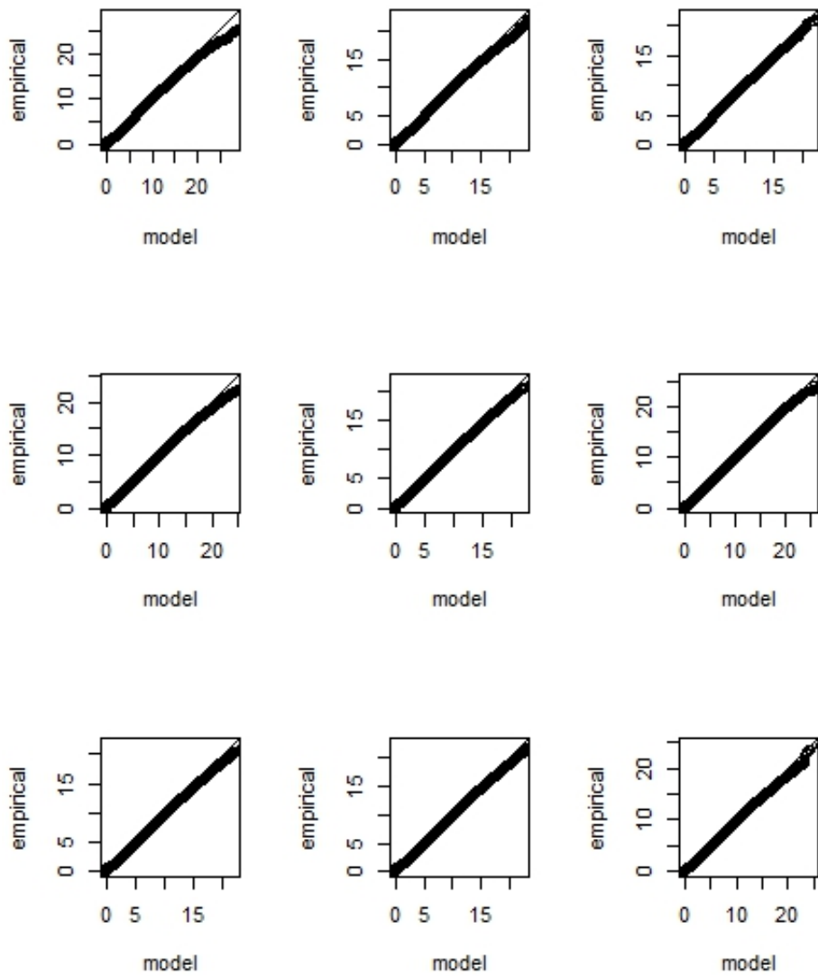
Figure 18: qq-plots of simulated vs. observed wind speed
