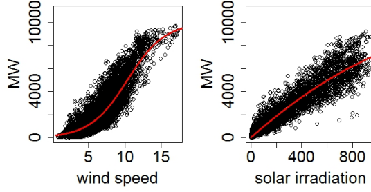
Figure 6: Empirical power curves
