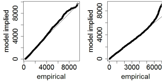
Figure 7: qq-plots of renewable generation
