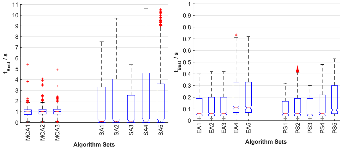
Fig. 9. Time to best-found solution comparison
