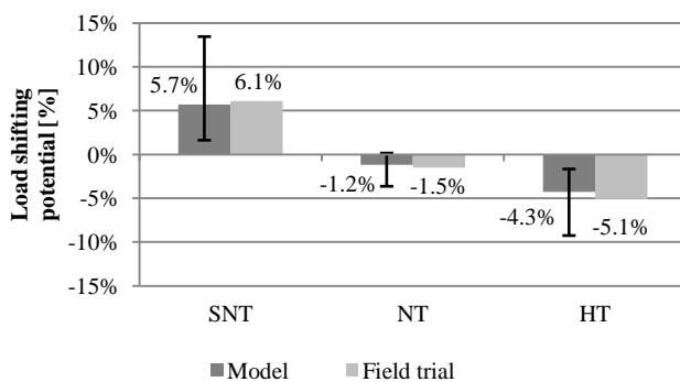
Fig. 3 Comparison of the modeled load shifting potential to the results from a field trial (cf. Hillemacher, 2014)
