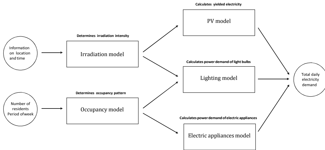
Figure 2.1.: Simplified overview of the models implemented in CREST.
