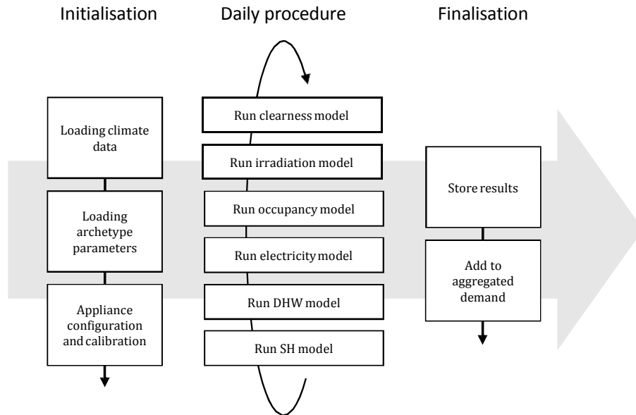
Figure 3.1.: Overview of the functions activated during a full year simulation process.
