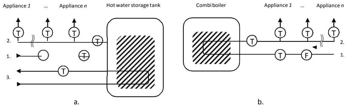
Figure 3.5.: Measurement setup for a. conventional boiler and b. combi boiler showing 1. cold feed inflow, 2. hot water pipe to appliances and 3. primary circuit to boiler (modified Figure from EST (2008)). 'T' indicates a temperature measurement point, 'F' indicates a flow measurement point.
