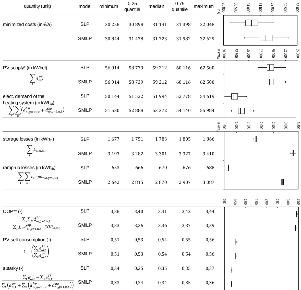
Fig.6: Characteristic values and measures of dispersion of 100 scenarios for the optimal solution of SLP and SMILP for building group 1, also shown as box-and-whisker (the whiskers represent the minimum and maximum of the values).
