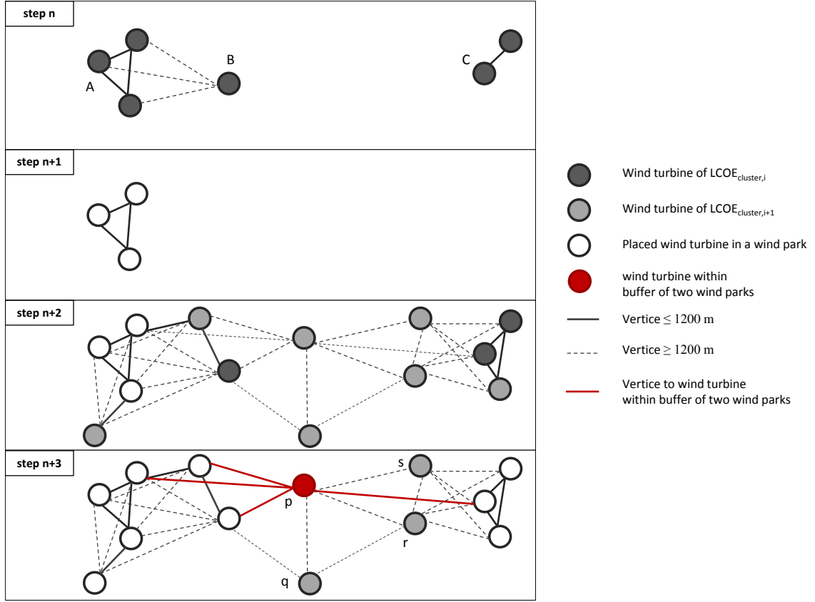
Figure 2: Algorithm to place wind parks.
