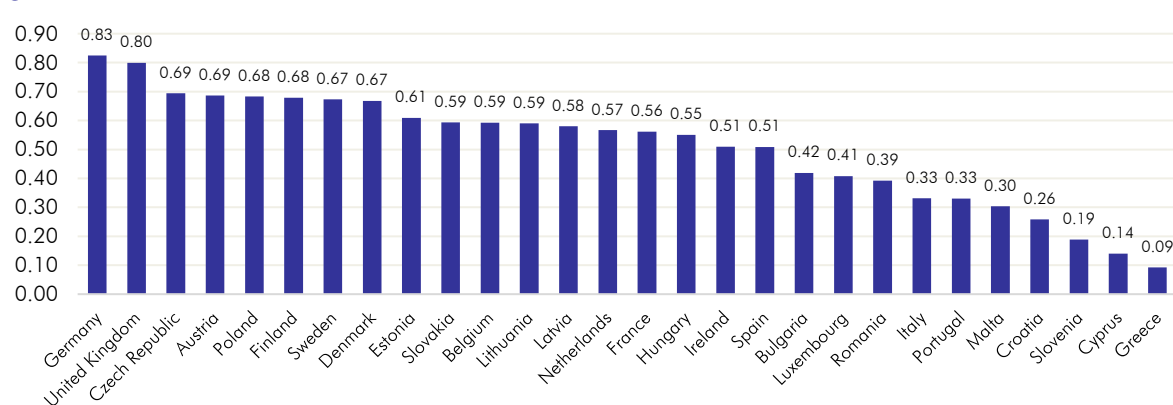
Figure A2.4: Macro subindex
