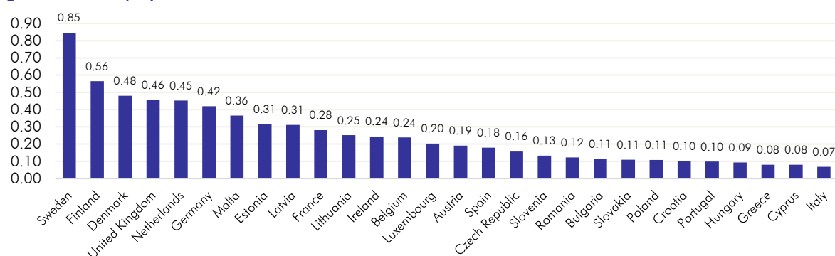
Figure A2.3: Equity subindex
