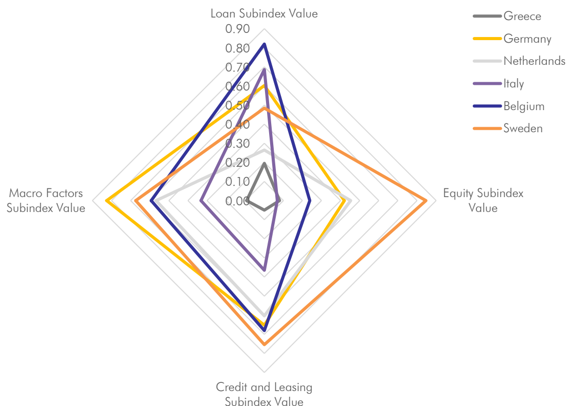
Figure 5: The 2016 ESAF subindices (examples for selected countries)
