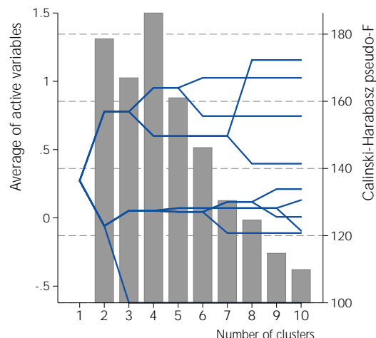
(b) Ward's method
