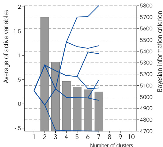
Figure F2: Clustergrams of different clustering methods
