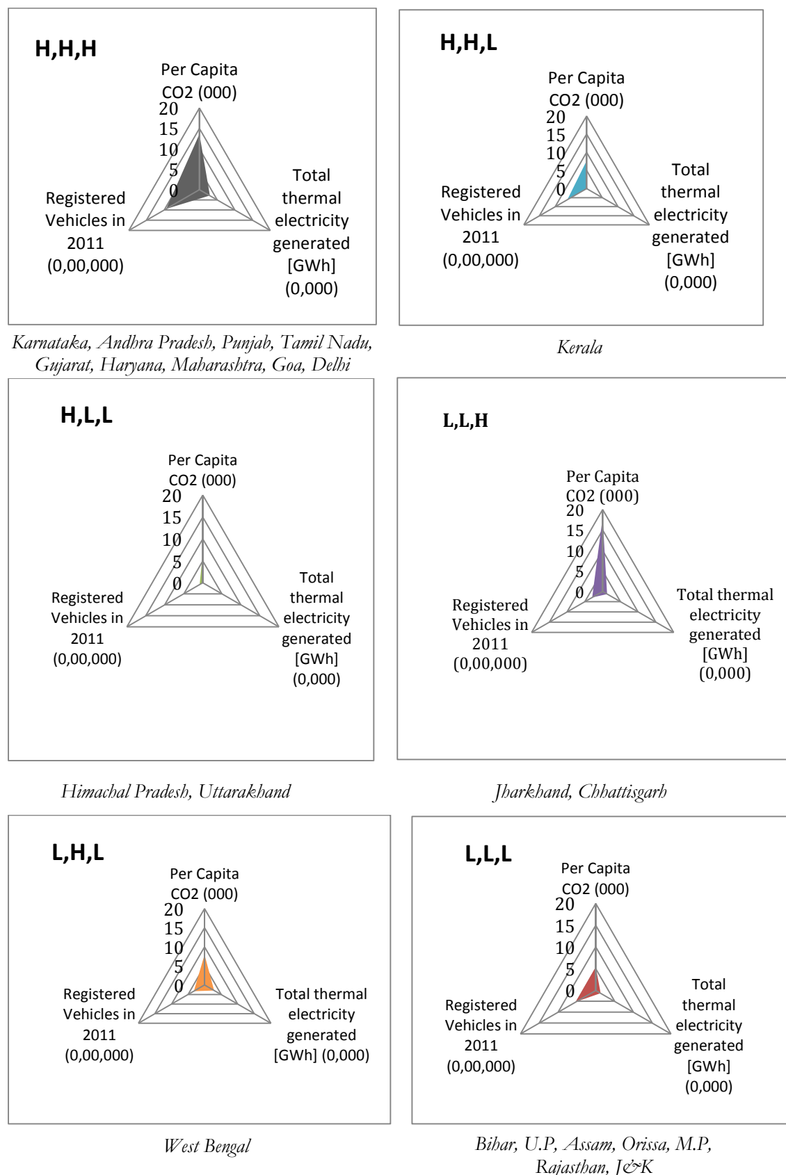
Figure 4: Carbon emissions and associated parameters for different state categories
