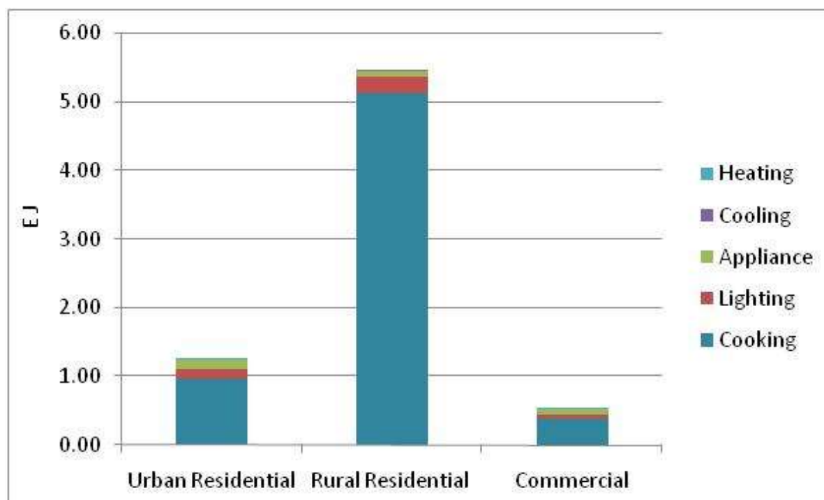
Figure 12: End-use energy demand in buildings
