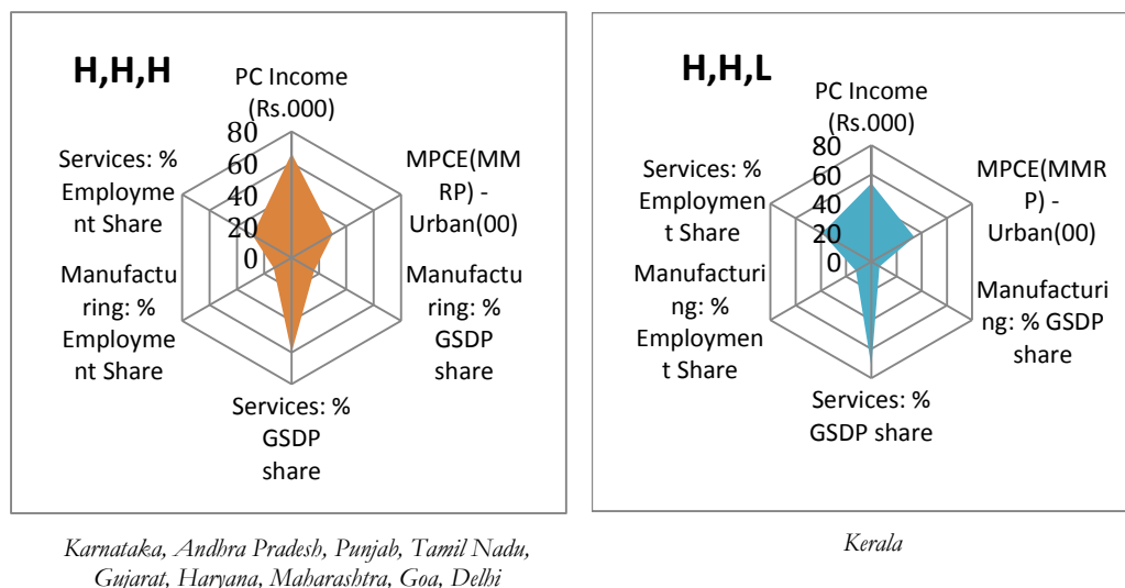
Figure 3: Income levels and associated economic parameters for different state categories
