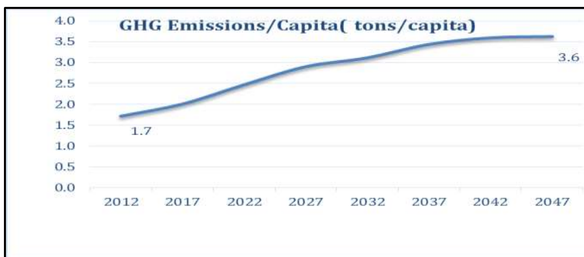
Fig 4.1: Emissions per capita in the Low Carbon Scenario
