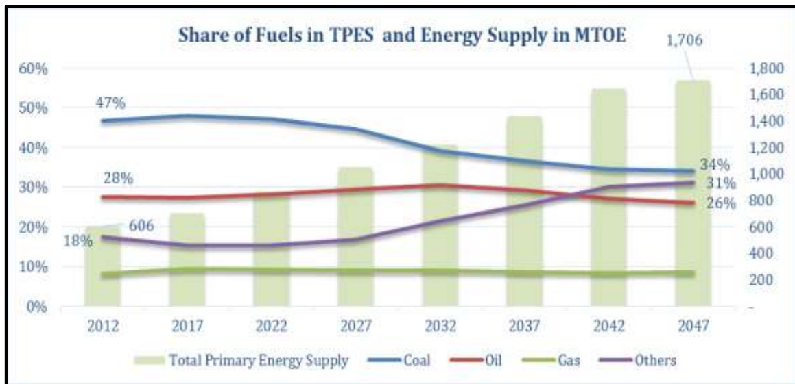
Fig 4.1.2: Composition of the Supply Sector in the low carbon scenario
