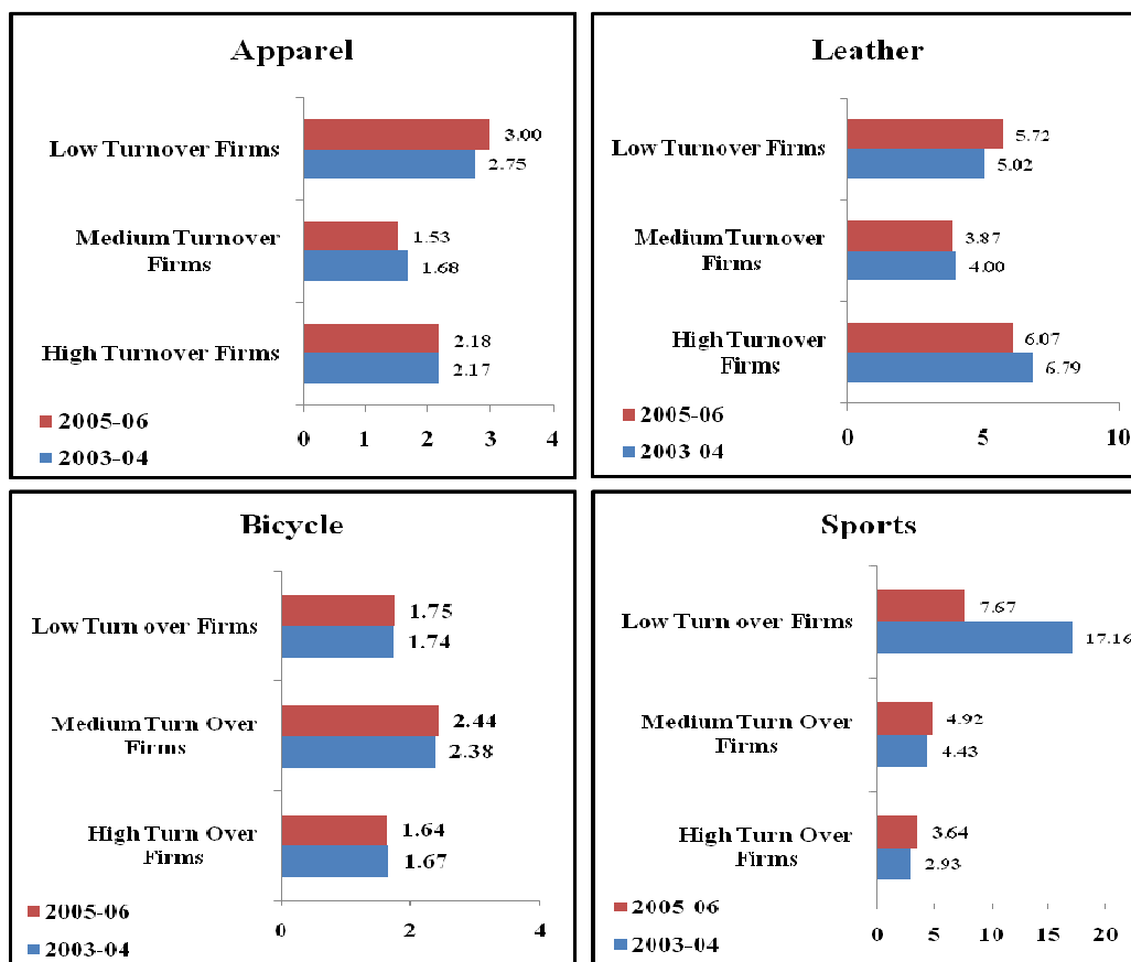
Chart 4: Change in Worker-Machine ratio during 2003-04 & 2005-06
