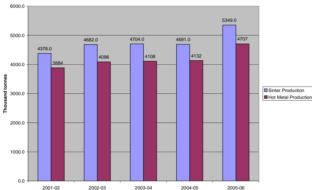
Sinter and Hot Metal Production : Bokaro SAIL
