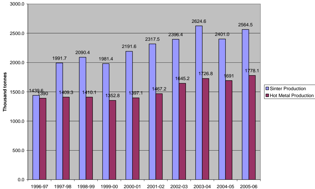
Sinter and Hot Metal Production :Rourkela SAIL
