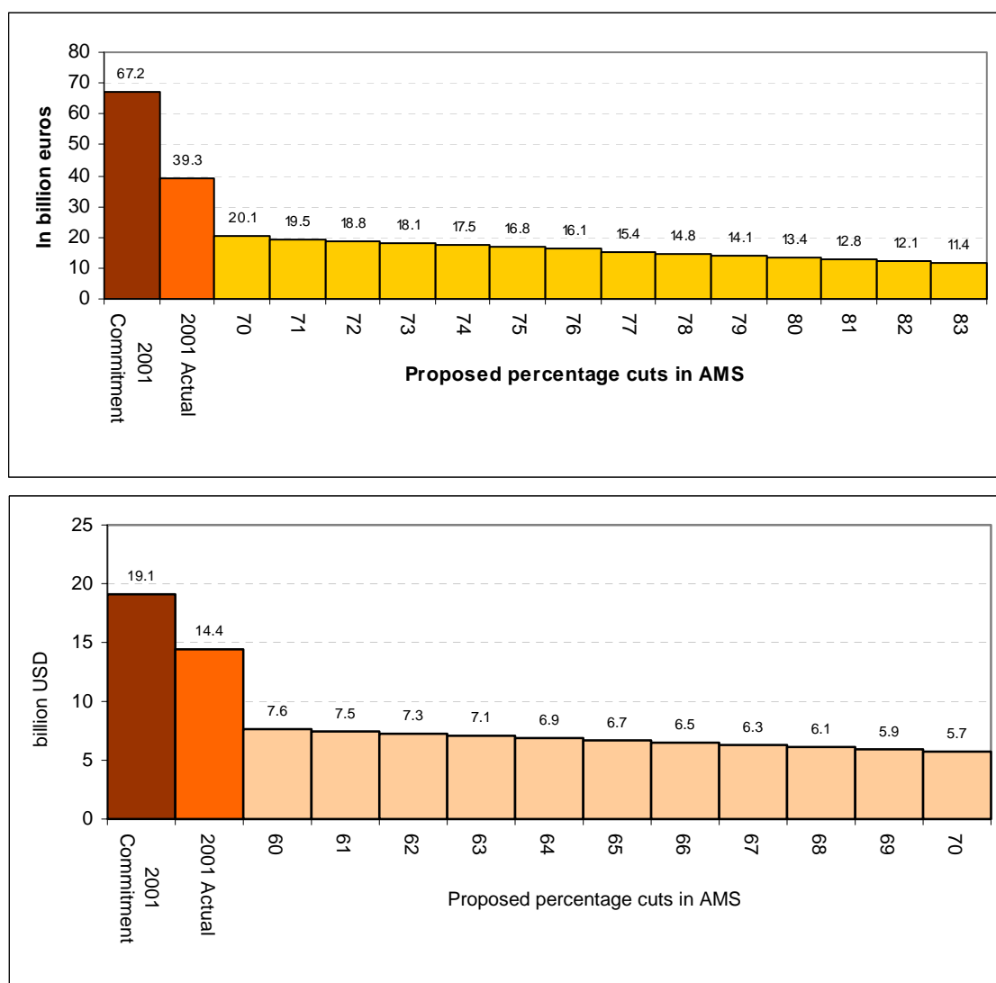
Figure 3.3. EU: Projected AMS levels after implementing the cuts proposed in the HK Draft Ministerial Text
