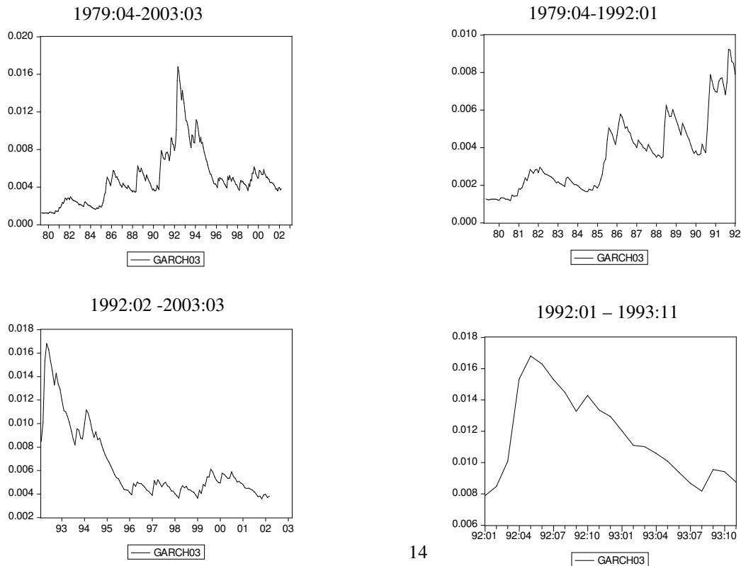
Fig. VI.1 Conditional Variance
