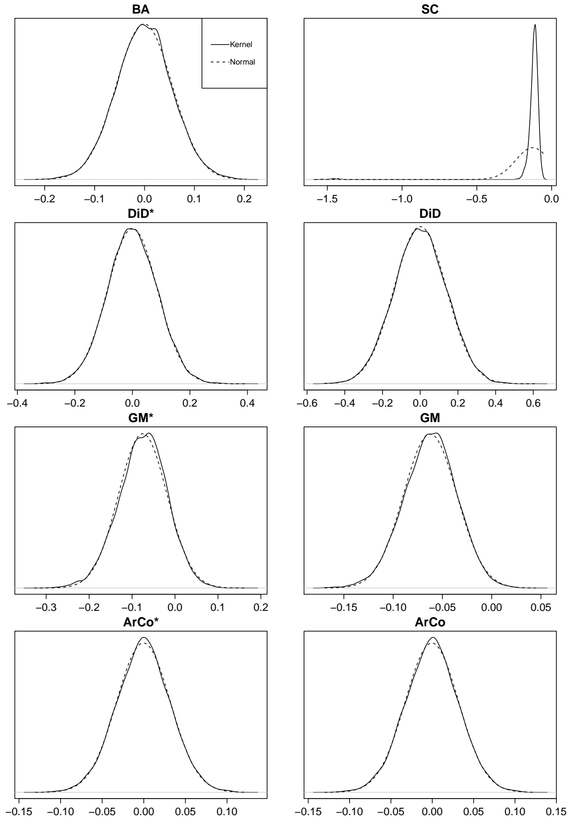
FIGURE 3. Kernel Density - Estimator Comparison with no Trend
