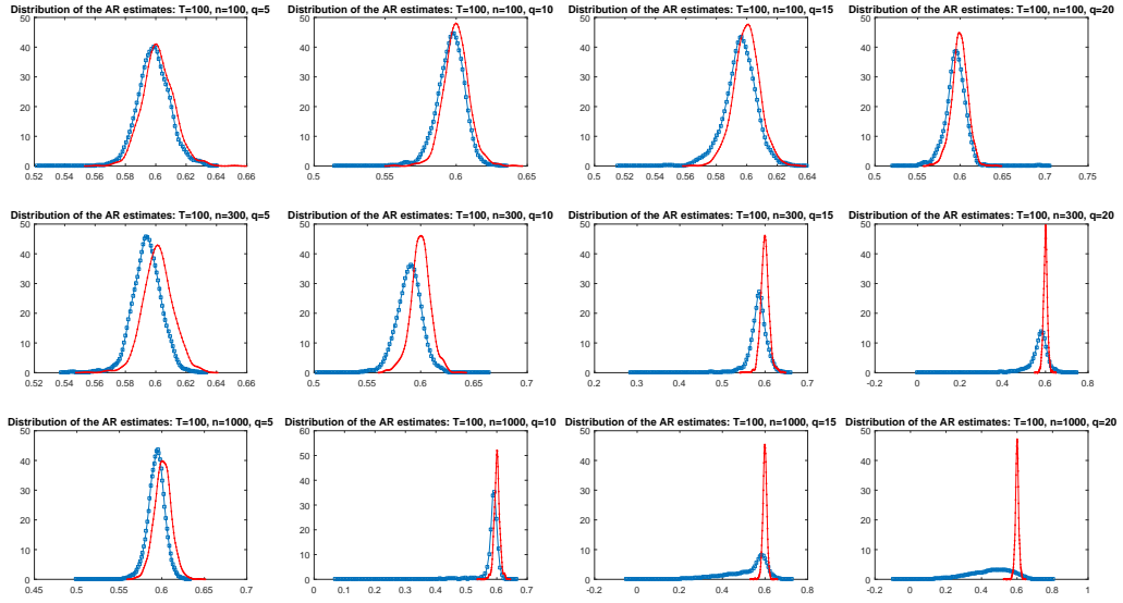
FIGURE 2. Distribution of the adaLASSO and Oracle estimators for the parameter \phi over 1000 Monte Carlo replications. Different combinations of candidate and relevant variables. The sample size equals 100 observations.
