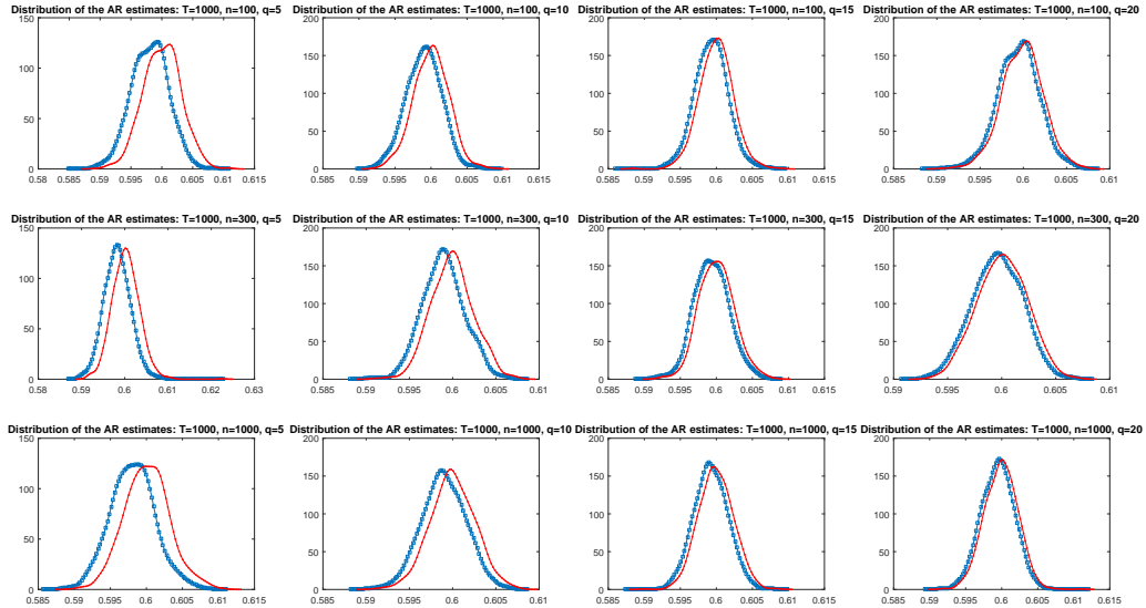
FIGURE 4. Distribution of the adaLASSO and Oracle estimators for the parameter \phi over 1000 Monte Carlo replications. Different combinations of candidate and relevant variables. The sample size equals 1000 observations.
