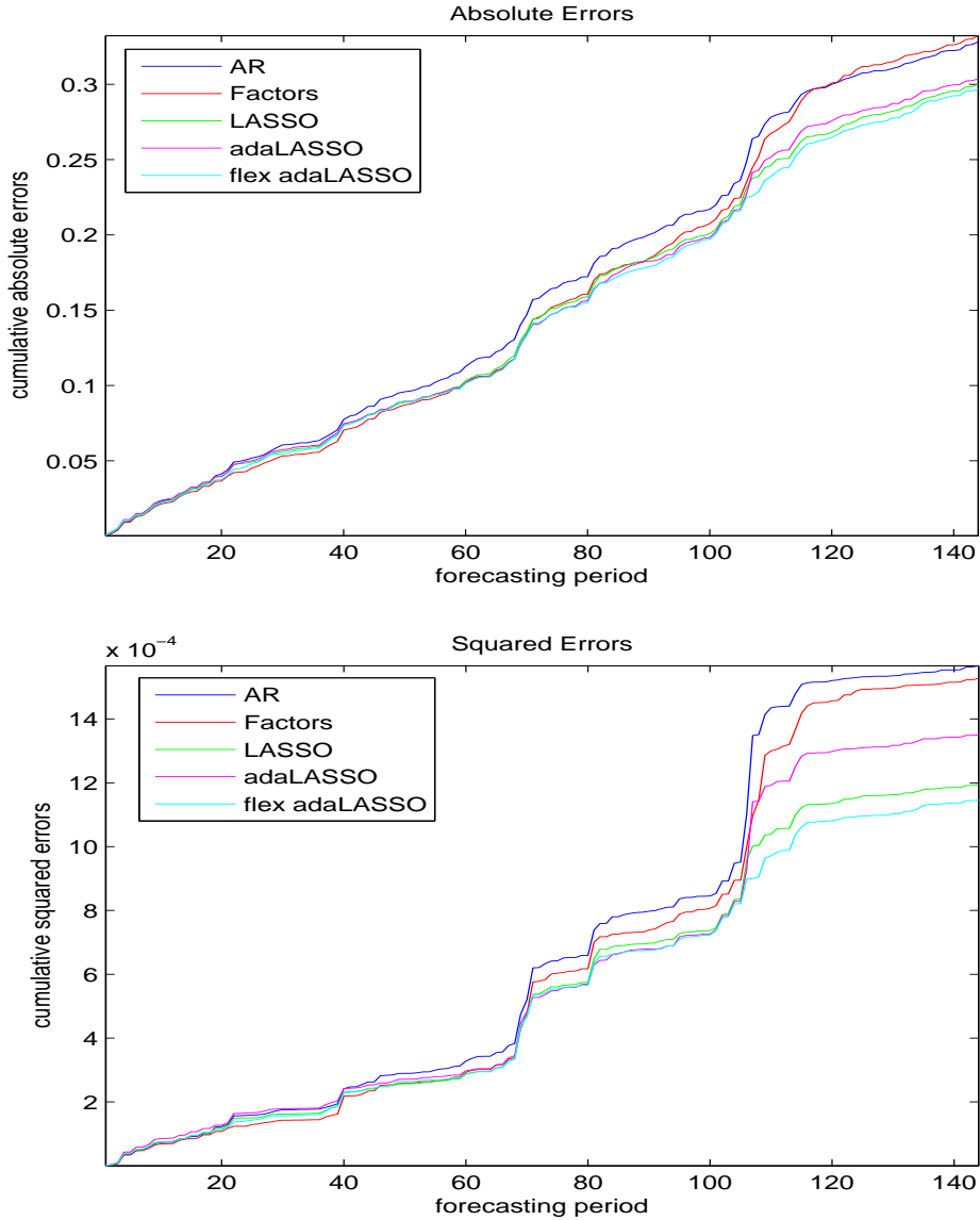
FIGURE 5. Panel (a): Cumulative absolute errors. Panel (b): Cumulative squared errors.
