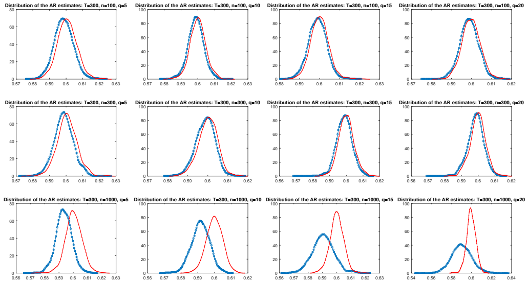
FIGURE 3. Distribution of the adaLASSO and Oracle estimators for the parameter \phi over 1000 Monte Carlo replications. Different combinations of candidate and relevant variables. The sample size equals 300 observations.
