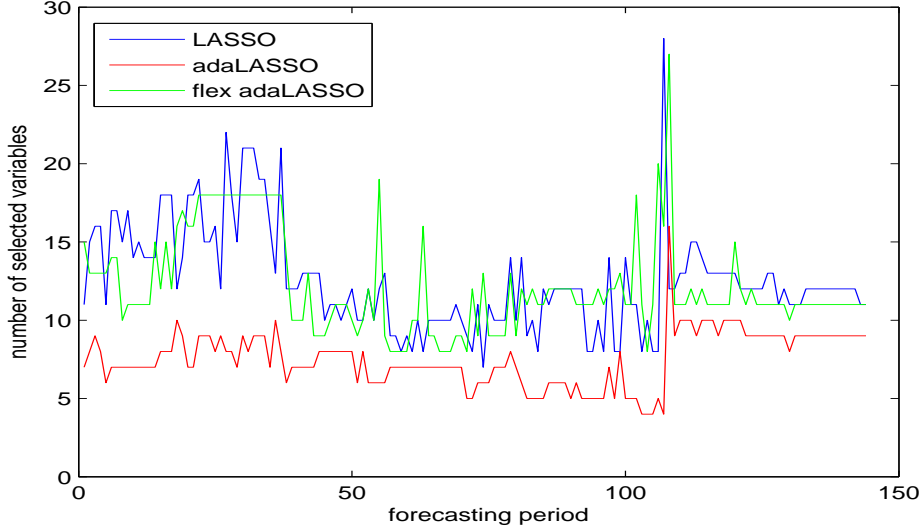
FIGURE 6. Number of parameters.
