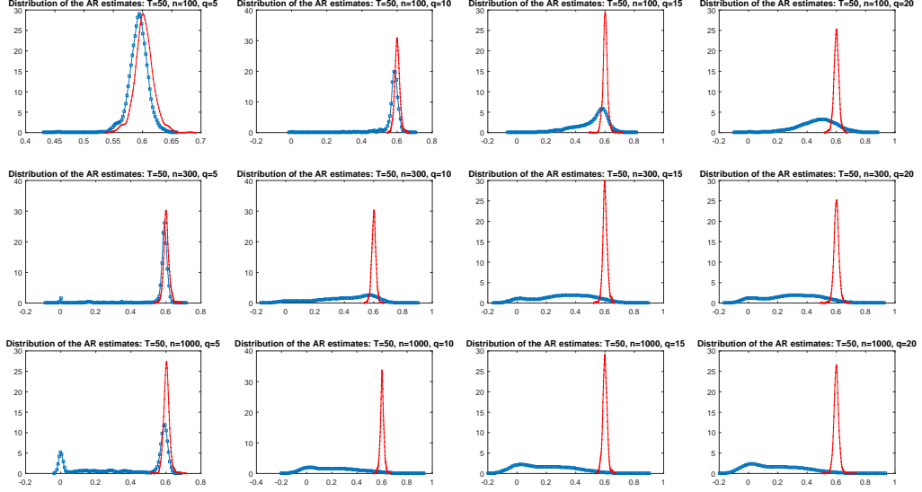
FIGURE 1. Distribution of the adaLASSO and Oracle estimators for the parameter \phi over 1000 Monte Carlo replications. Different combinations of candidate and relevant variables. The sample size equals 50 observations.
