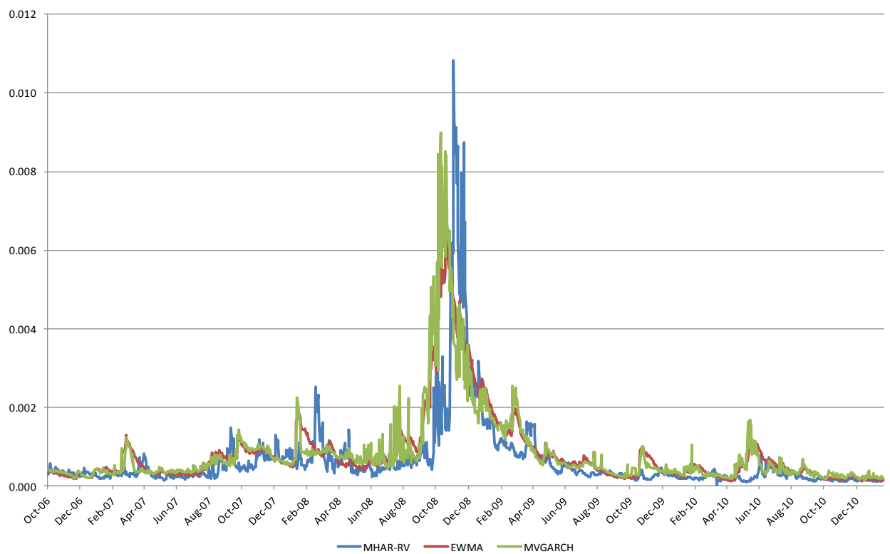
Graph 2: Daily volatility of Vale (VALE5) according to different forecasting models (EWMA, MVGARCH and MHAR-RV)
