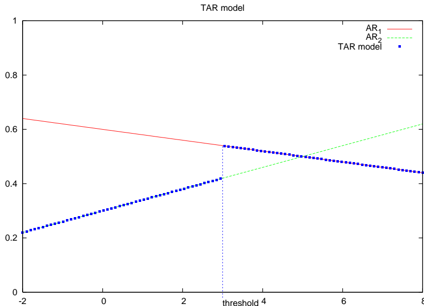
Figure 1: An example of TAR model
