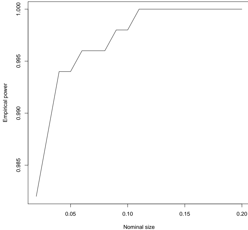
Figure 6: Empirical power versus nominal size for the linearity test applied on model (31).
