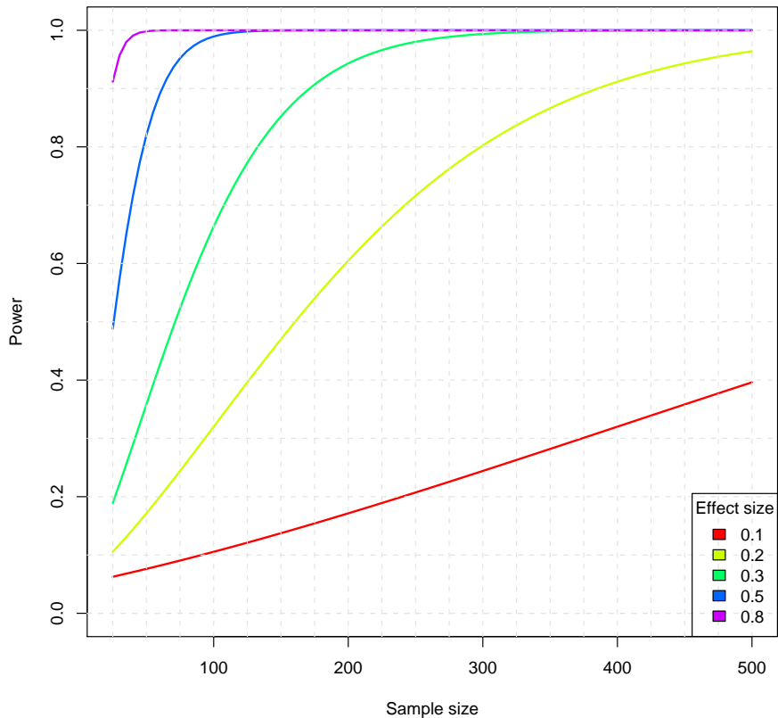
Figure 5: Power estimation for linearity test.
