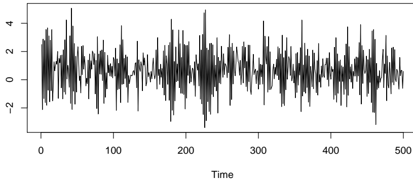
Figure 4: Generated series for model (26), stationary linear autoregressive model.
