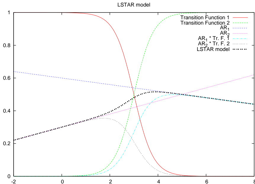
Figure 2: An example of 2 regime STAR model using logistic transition function.
