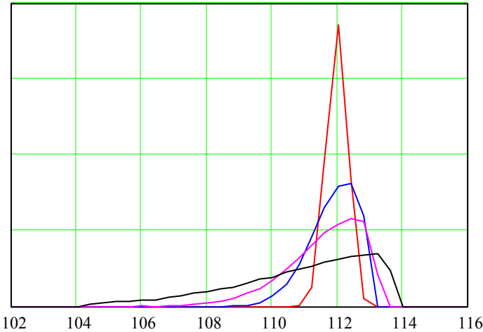
Figure 5.2 Distribution of the Level of the Aggregate Output in the End Period
