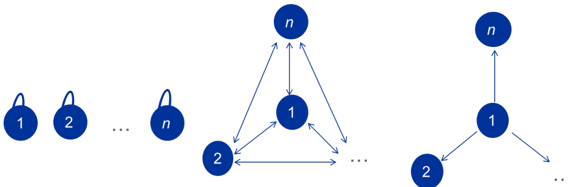
Figure 1: Stylised network representations
