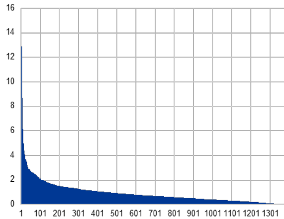
Figure 2: The weighted degree distribution across sectors
