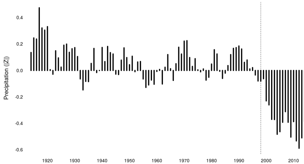
Figure 1: Precipitation patterns 1915-2014
