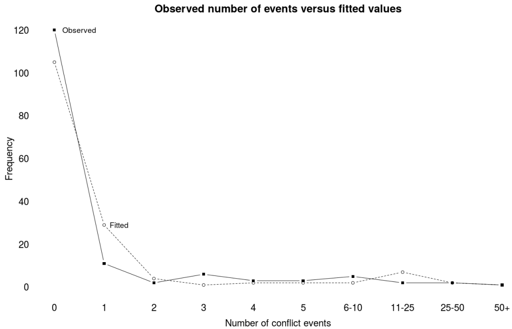
Figure 4: Marginal calibration diagram
