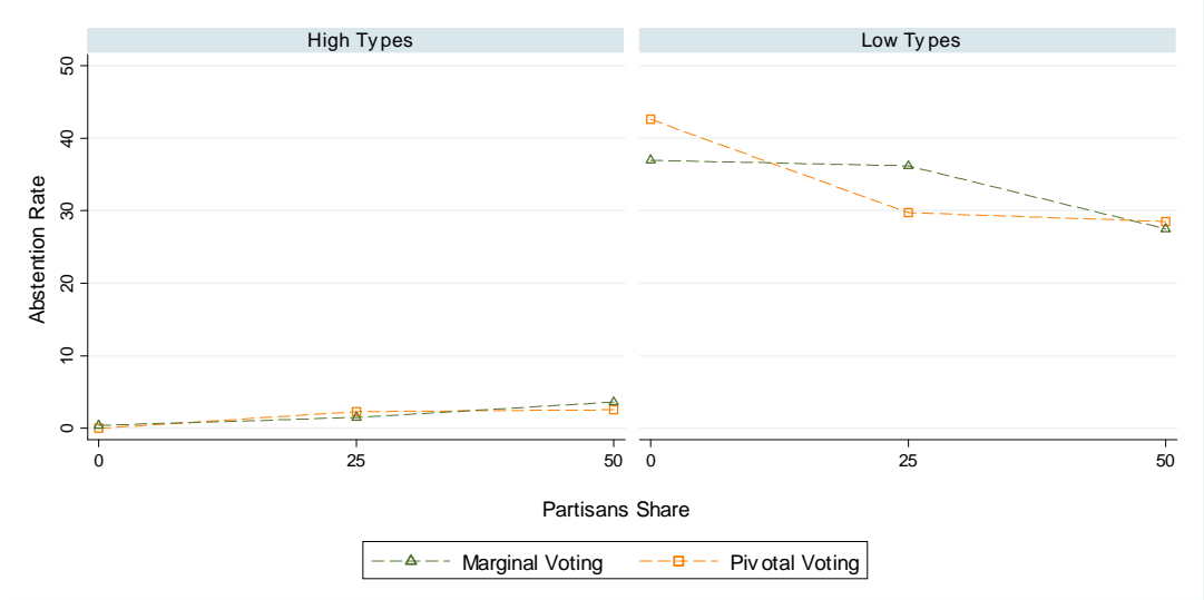
Figure 7: Observed abstention for each treatment, by voter type, averaged across round and groups.
