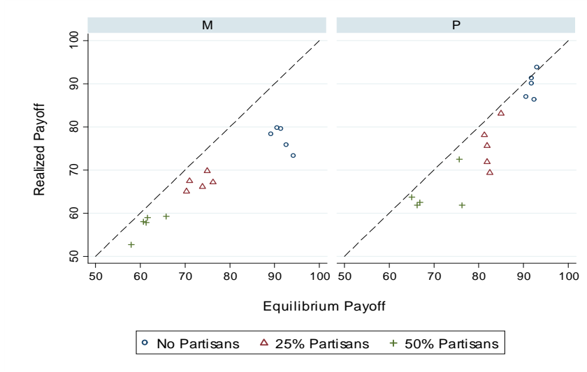
Figure 8: Realized payoff vs equilibrium payoff in each independent group.
