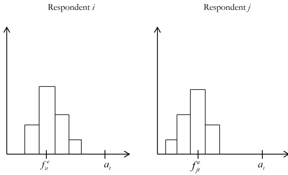
Figure 2. Motivating a Density Accuracy Measure
