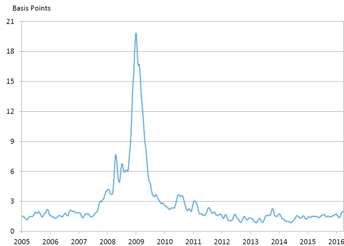
Figure 22: Spline Errors of U.S. Treasury Securities
