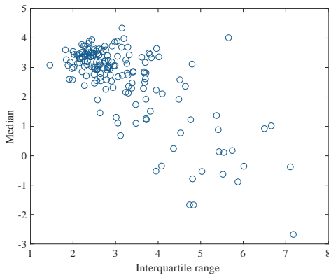
(c) Q5 and Interquartile Range One quarter ahead
