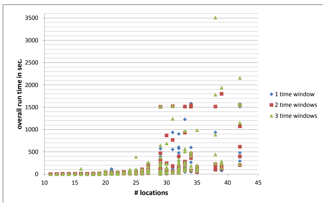
Figure 21: Run times depending on the number of locations and the number of time windows
