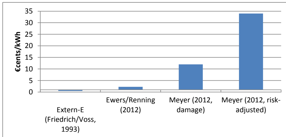
Figure 1: Estimates of the long-run social external costs of nuclear power
