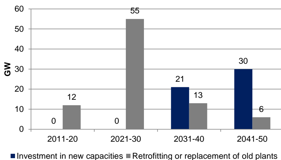
Figure 3: New-built and retrofit nuclear power plants in the EU 2016 Reference Scenario
