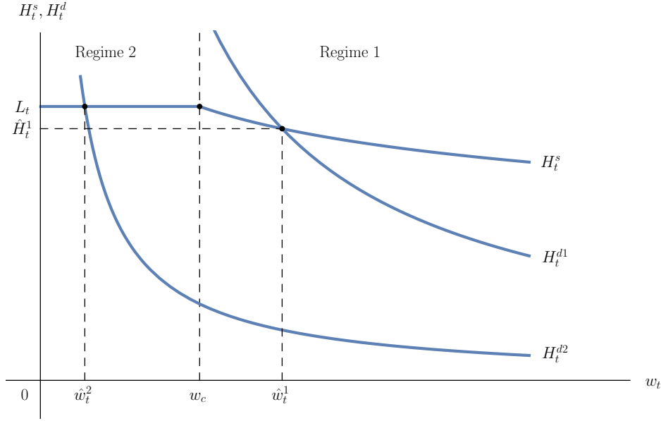
Figure 3.1: The labor market equilibrium of period t . If the aggregate demand for hours worked is H_t^{d1} then the labor market equilibrium is (\hat{w}_t^1, \hat{H}_t^1) . The individual supply of hours worked is in Regime 1, i. e., it falls in w_t , and aggregate demand for hours worked is high. If the aggregate demand for hours worked is H_t^{d2} then the labor market equilibrium is (\hat{w}_t^2, \hat{H}_t^2) where \hat{H}_t^2 = L_t \cdot 1 . The individual supply of hours worked is in Regime 2, i. e., it does not hinge on w_t , and aggregate demand for hours worked is low.
