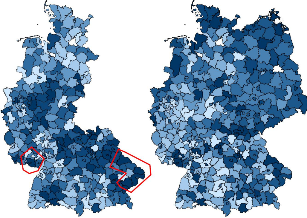
Figure A1: T_{it} in 1987–1998 (Left), and 1998–2009 (Right)
