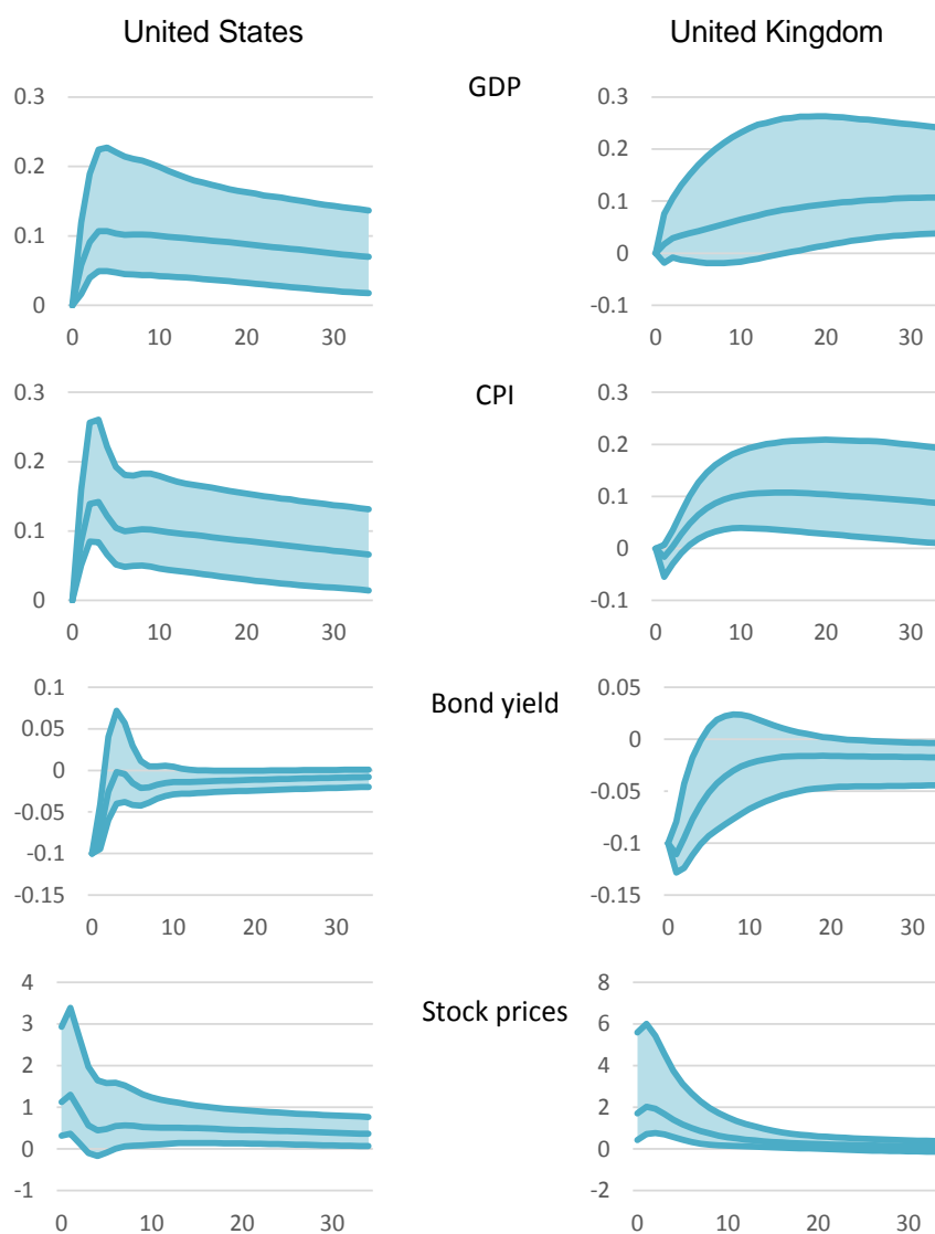
Figure 6: Impulse responses to a term spread shock (full sample)
