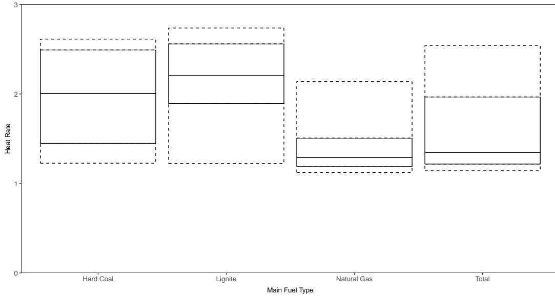
Figure 5: Distribution of Average Actual Measured Heat Rates in 2003 and 2004
