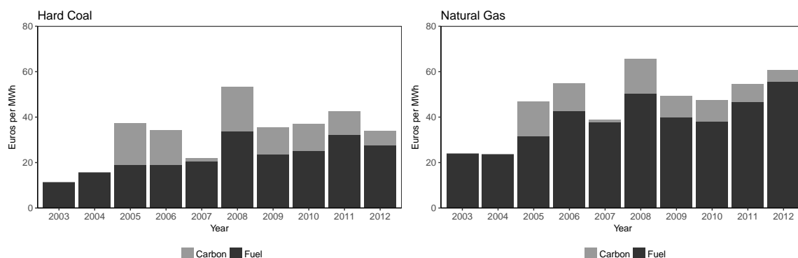
Figure 1: Average Fuel and Carbon Cost in Power Generation
