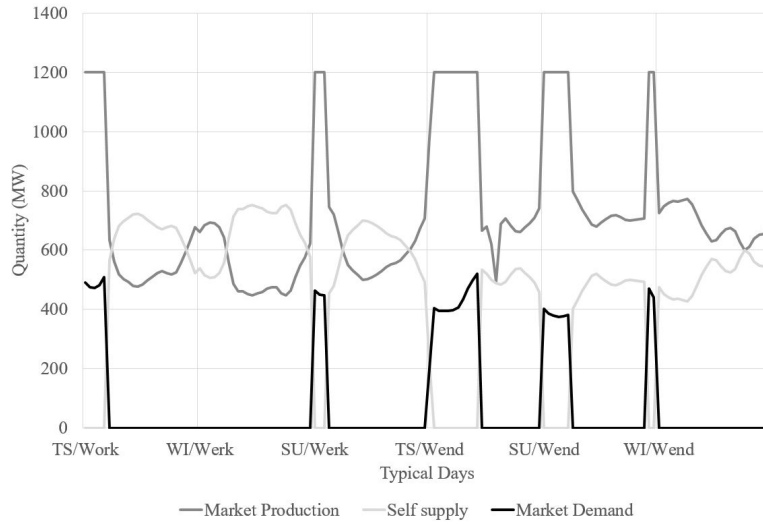
Figure 7: Optimal Prosumer Decisions for Production Capacity of 1200 MW and Production Costs of 10 EUR/MWh
