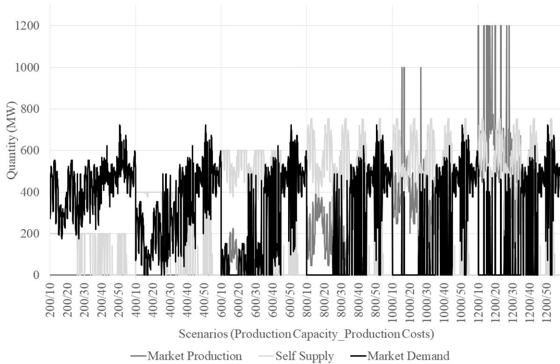
Figure 14: Optimal PS Decisions for 4,320 Typical Hours
