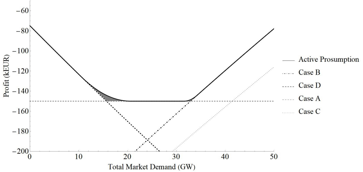
Figure 4: Profit Comparison with Changing Total Market Demand Q_d^{market}
