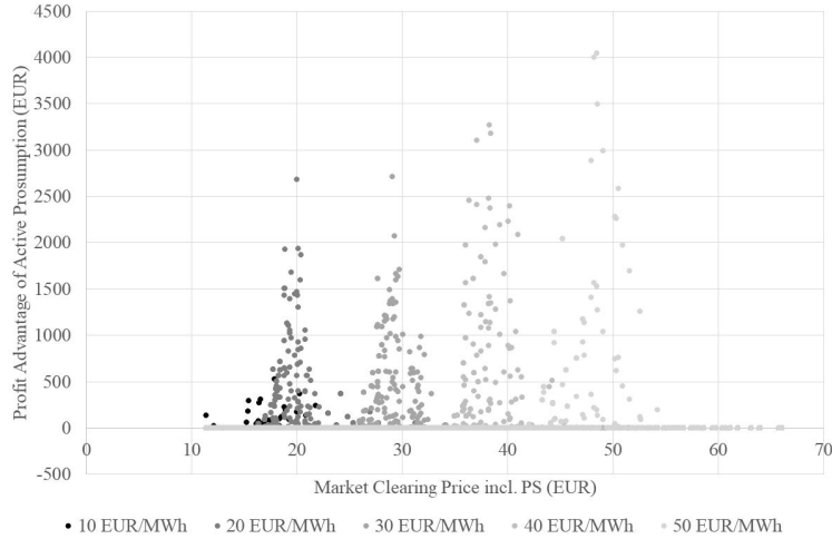
Figure 13: Profit Advantage of Active vs. Passive Prosumption
