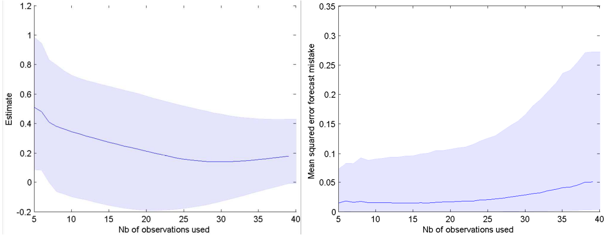
Figure 6: Cross-sectional performance across agents using different number of observations required to perform RLS. Left: Binned plot relating sample size and estimated coefficients. Right: Binned plot relating sample size and demand forecast mistakes.
