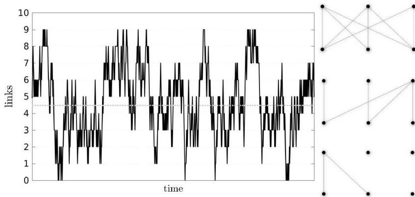
Figure 3: Left: An example of a small network with N = 10 nodes at criticality (i.e., \Delta = 0 ). Right: Example states of the system with N_1 = N_0 = 3 , showing highly connected, intermediate, and sparsely connected states.
