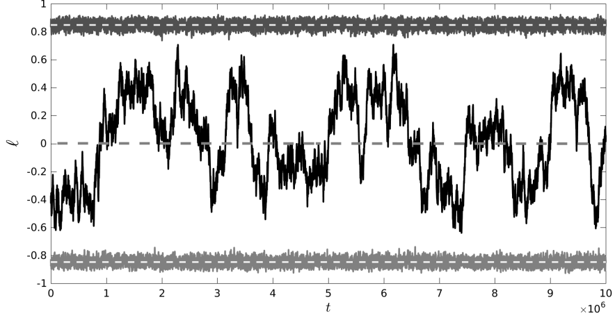
Figure 2: Three different trajectories of the connectance \ell for three different values of the population parameter \Delta . The top dark gray time series is the case \Delta = 0.1 , the central black time series is for the critical value of \Delta = 0 , the bottom light gray series is for \Delta = -0.1 . The dashed horizontal line is the zero connectance, Above this line the system is in a dense network state, below the line the system is in a sparse network state. The dashed horizontal lines represented the average values as predicted by the analytical calculations.
