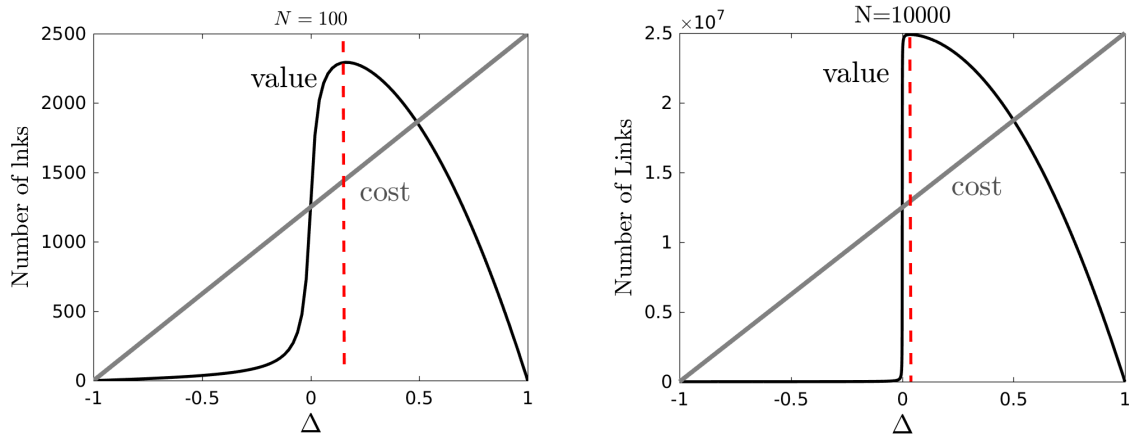
Figure 8: We see how the maximum profit is obtained for value of \Delta that tend to the critical point as N \rightarrow \infty . In this case we took \alpha = N/4 to compare the two graphs. The largest distance between the value curve and the cost curve is point of the maximum profitability. The value curve has been plot using the analytical prediction as in eq.(14).
