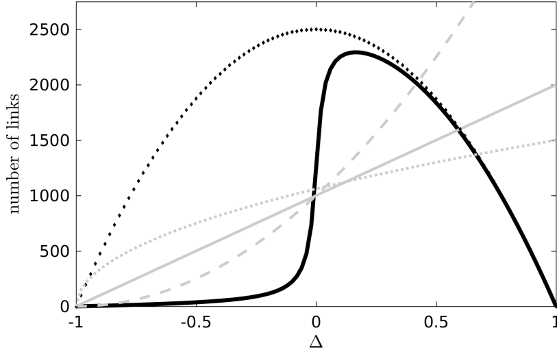
Figure 9: Example of non-linear cost functions. The profitable region changes and the \Delta_{max} shifts according to shape of the cost function which can have any generic shape according to a specific context. In the figure, the gray curves represent various cost functions. To keep the curves consistent we have arbitrarily chosen the linear cost function as \frac{N}{5}N_1 , the quadratic cost function as \frac{N}{25}N_1^2 , and the square root cost function as \frac{3N}{2}\sqrt{N_1} . On the other side, the black curves represent the values of the network. The bold one corresponds to the actual created links as by eq.(5), whereas the dotted black line is the number of the potential links N_0N_1 = N^2(1 - \Delta^2)/4 which has its maximum value at \Delta = 0 for any system size N .
