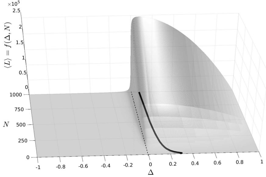
Figure 6: A three dimensional plot of the expected number of links as a function of the scaled population difference \Delta and the system size N . The black curve in the horizontal plane represents the loci of maximum points, S(N) , for which we have the highest number of links for each system size. We see that for small networks the maximum point is in the super-critical regime ( \Delta > 0 ), as the network size increases the maximum points tend asymptotically to the critical value of \Delta = 0 .
