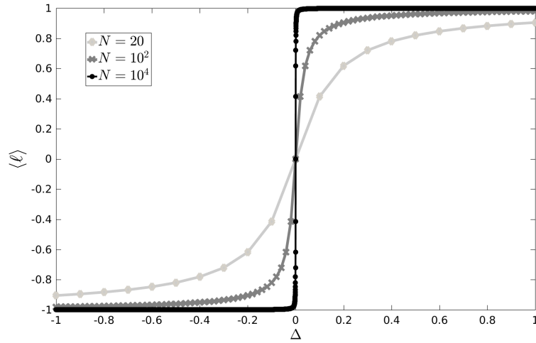
Figure 4: Finite size effects on the equilibrium value of the connectance.
