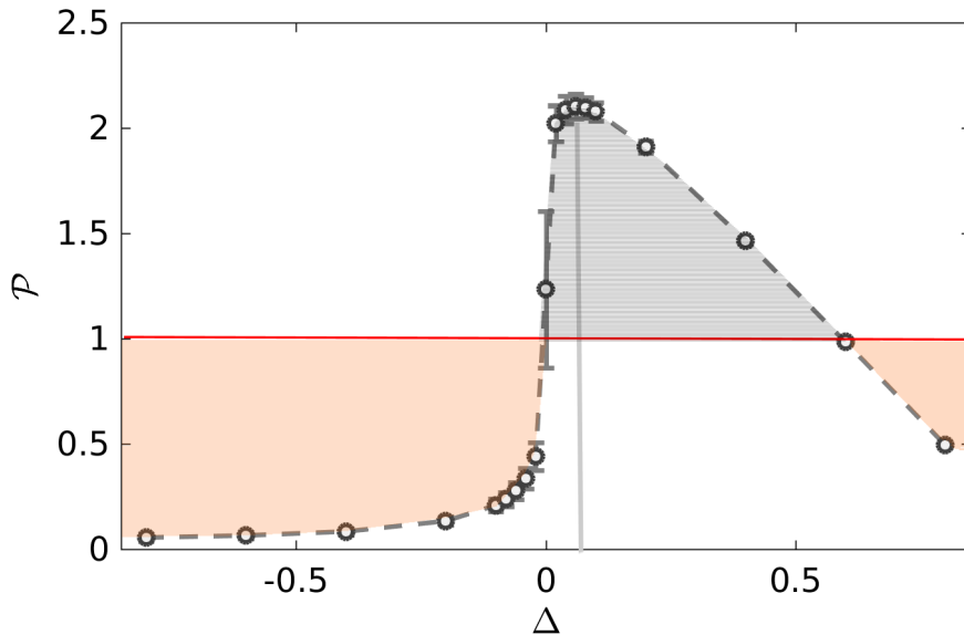
Figure 7: Profitability of a network with N = 100 total nodes in a Monte Carlo simulation. The horizontal line represent the profitability threshold. For the points which are below the line the system is in an unprofitable state. Above the line, the system can be profitable since \mathcal{P} > 1 . The shaded-striped area represents the interval for which the network is profitable in this specific case of linear cost. The vertical line indicates the point of maximal profitability \Delta_{min} . The error bars represent the uncertainty of the profitability since the system undergoes fluctuations due (in our mode) to the linking variance and are of the order of \sigma(\mathcal{P}) = \sigma(\ell)N_0/2\alpha . So, at criticality \mathcal{P} has the largest uncertainty and in our example this means that the network goes through unprofitable periods during its temporal evolution. During those times the system can be more vulnerable to losses, for example, by external shocks.
