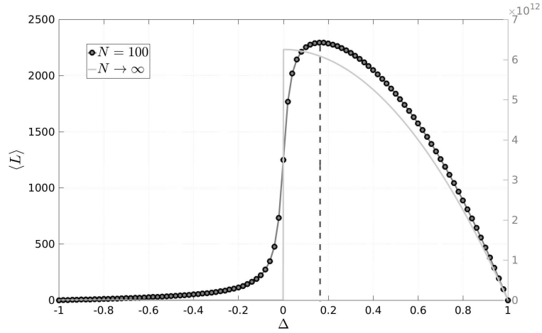
Figure 5: Average number of actualized links in a network with N = 100 units, dotted dark gray points. We observe how the maximum number of links is obtained for \Delta > 0 (located at the dashed line), so the maximum point is not the critical point as in the case of an infinite network (here 1 million nodes) represented by the light grey curve.
