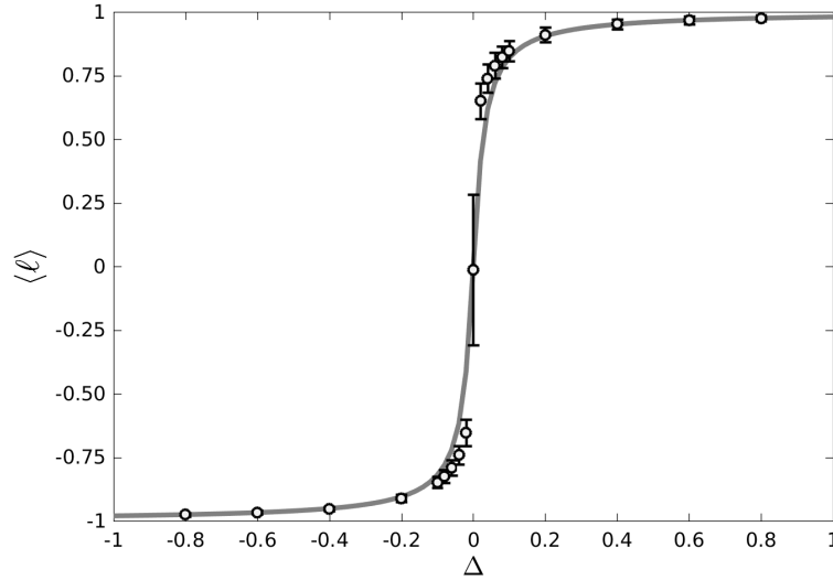
Figure 1: The average connectance as a function of the scaled population difference \Delta . The solid gray line represents the prediction of eq.(11). The points come from the results of monte carlo simulations, with error bars indicating the standard deviation. This figure was done with N = 100 nodes.
