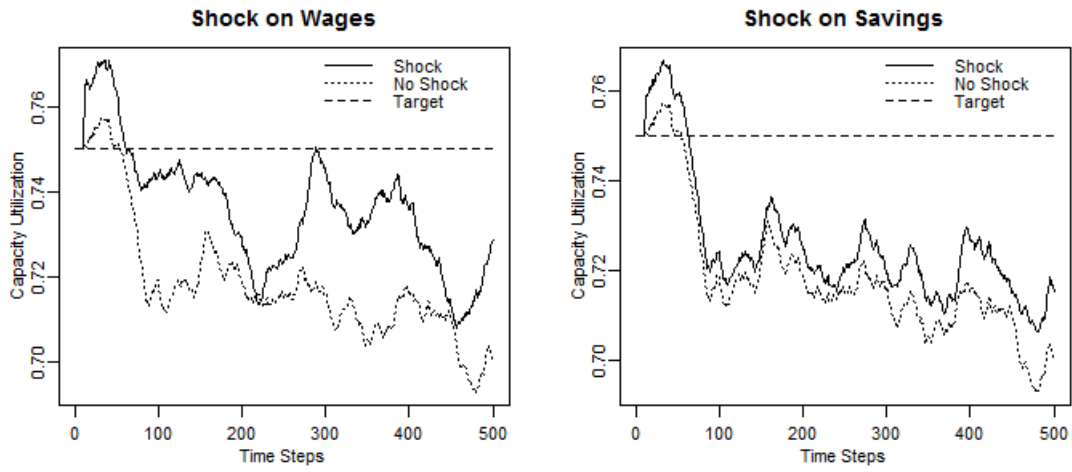
Figure 5: Capacity utilization evolution (single realization) - Shock vs. No shock scenarios
