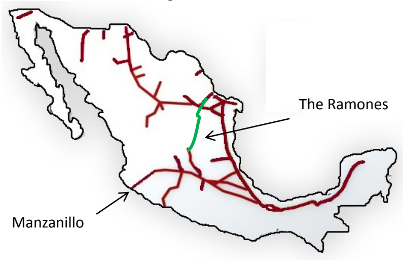
Figure 8 National Gas Pipeline System Proposed Scheme
