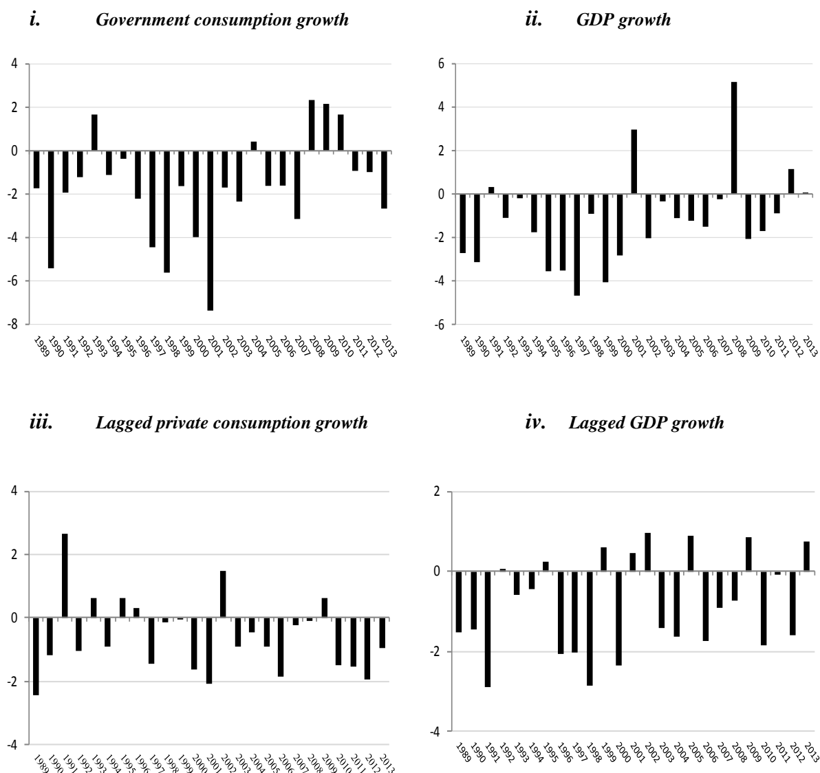
Figure 2. Forecast Errors, 1989-2013 (%)
