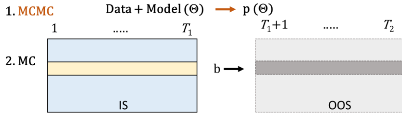
Figure 4. Two step Bayesian simulation (MCMC parameter estimation and MC data simulation)
