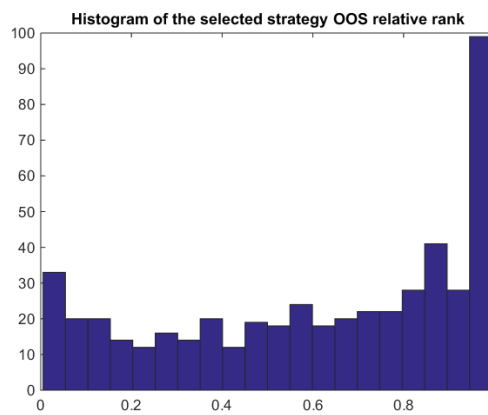
Figure 15. Bayes model 2 histogram of the out-of-sample relative rank of the best IS strategy
