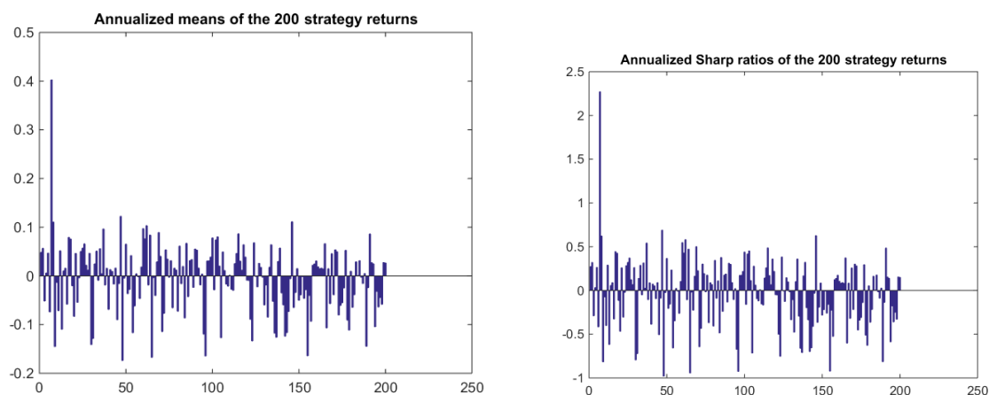
Figure 18. The modified annualized mean returns and Sharp ratios
