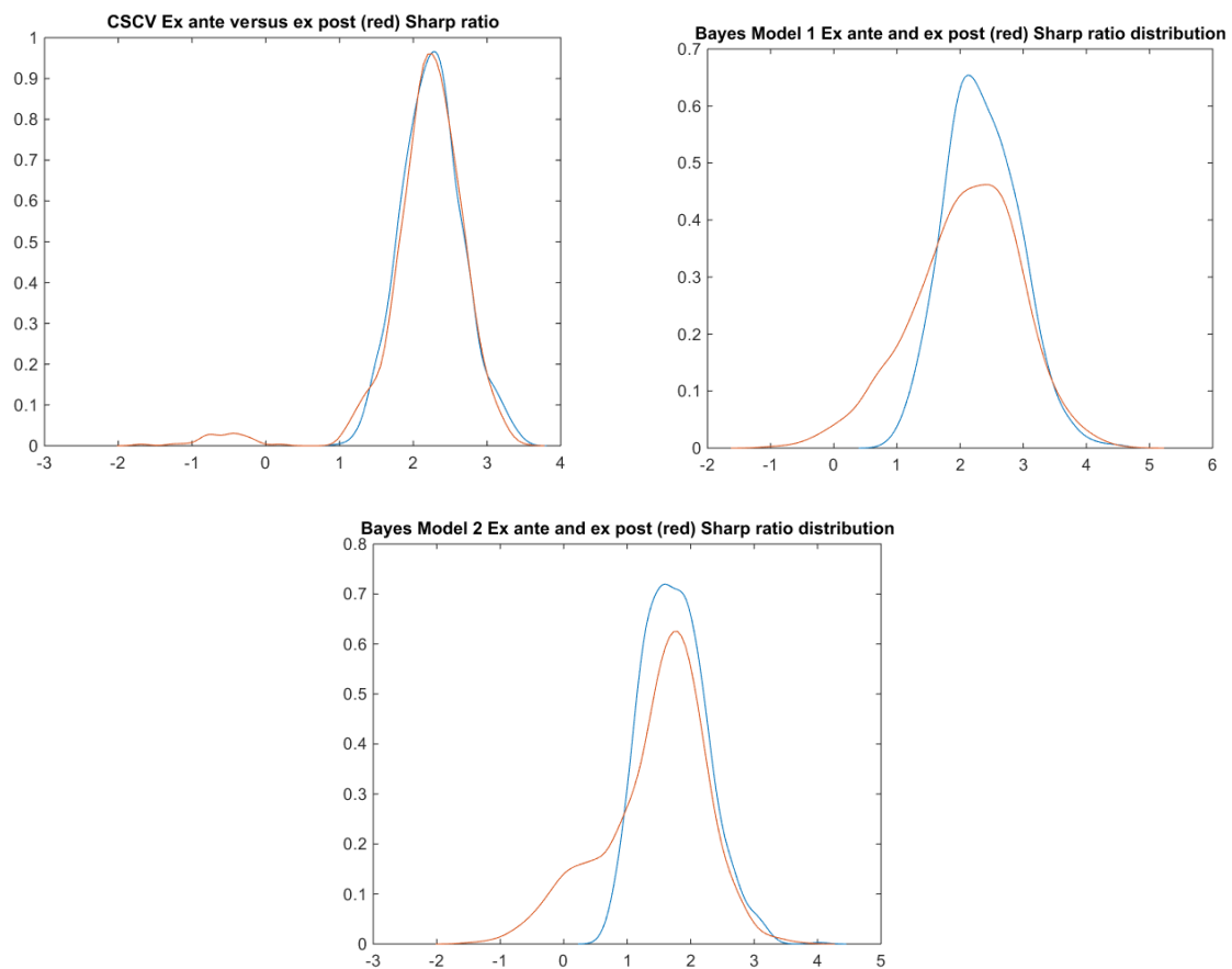
Figure 19. The simulations of the ex-ante and ex post SR densities
