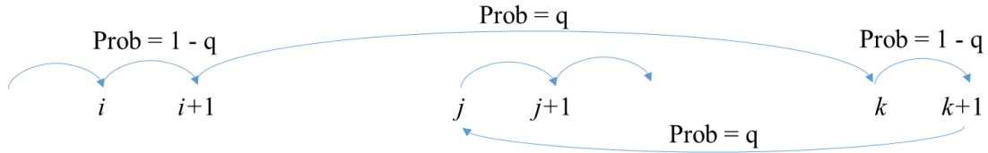
Figure 2. Stationary Bootstrap Process
