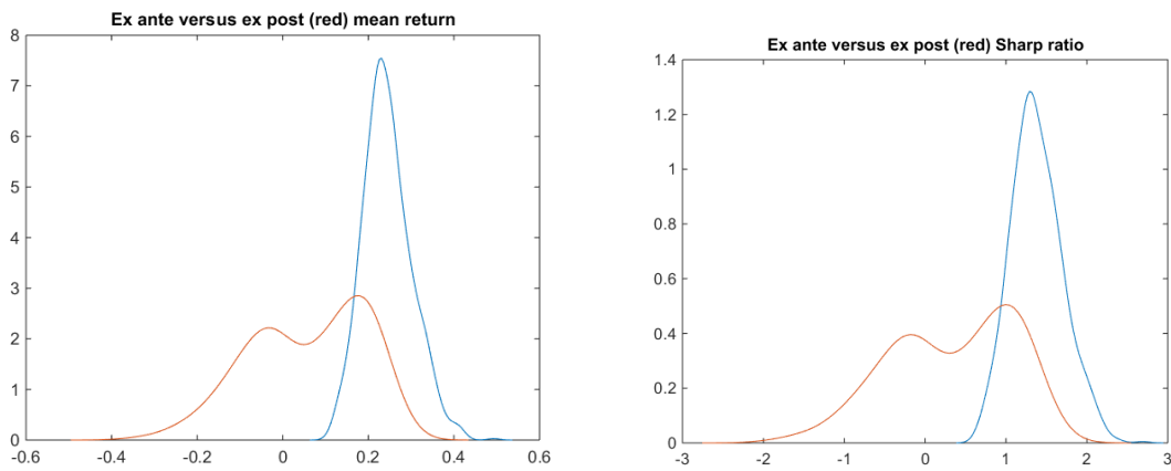
Figure 10. CSCV simulation of the ex-ante and ex post densities
