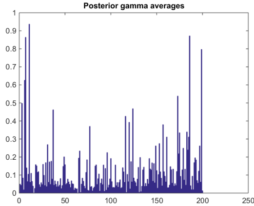
Figure 16. Posterior gamma average values for the 200 strategies
