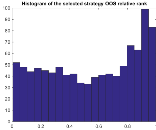
Figure 9. Histogram of the out-of-sample relative rank of the best IS strategy
