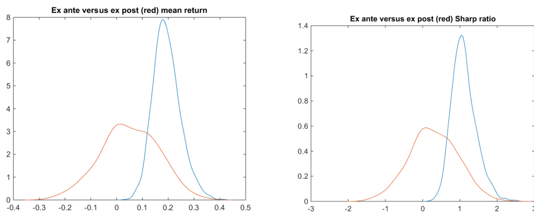
Figure 8. Sharp ratio and the mean return ex ante and ex post densities
