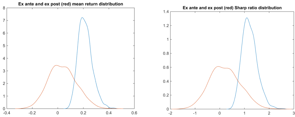
Figure 14. Bayes model 2 simulation of the ex-ante and ex post densities
