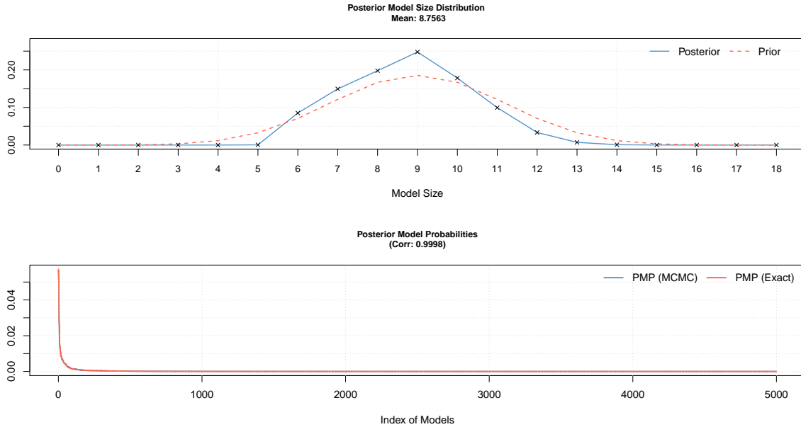
Figure 8: Model size and convergence of main BMA estimation
