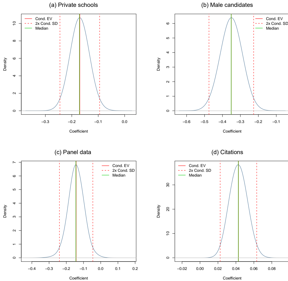
Figure 7: Posterior coefficient distributions for the most important characteristics
