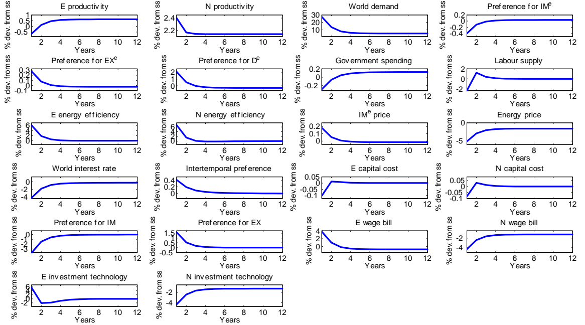
FIGURE V: IMPULSE RESPONSES OF OUTPUT TO THE SHOCKS.
