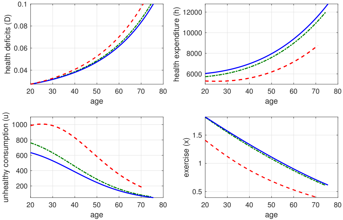
Blue (solid) lines: Reference American. Red (dashed) lines: untreated depressed individual ( \delta = 1.74, \eta = 0 ). Green (dash-dotted) lines: treated depressed individual ( \delta = 1.74, \eta = 0.0003 ).
