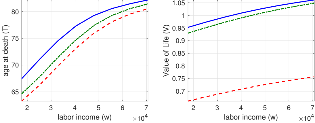
FIGURE 4: INCOME GRADIENT ( \phi_m = 1 )
