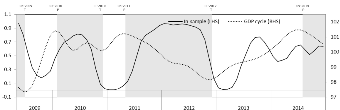
Figure 2 Estimated probabilities and the GDP cycle
